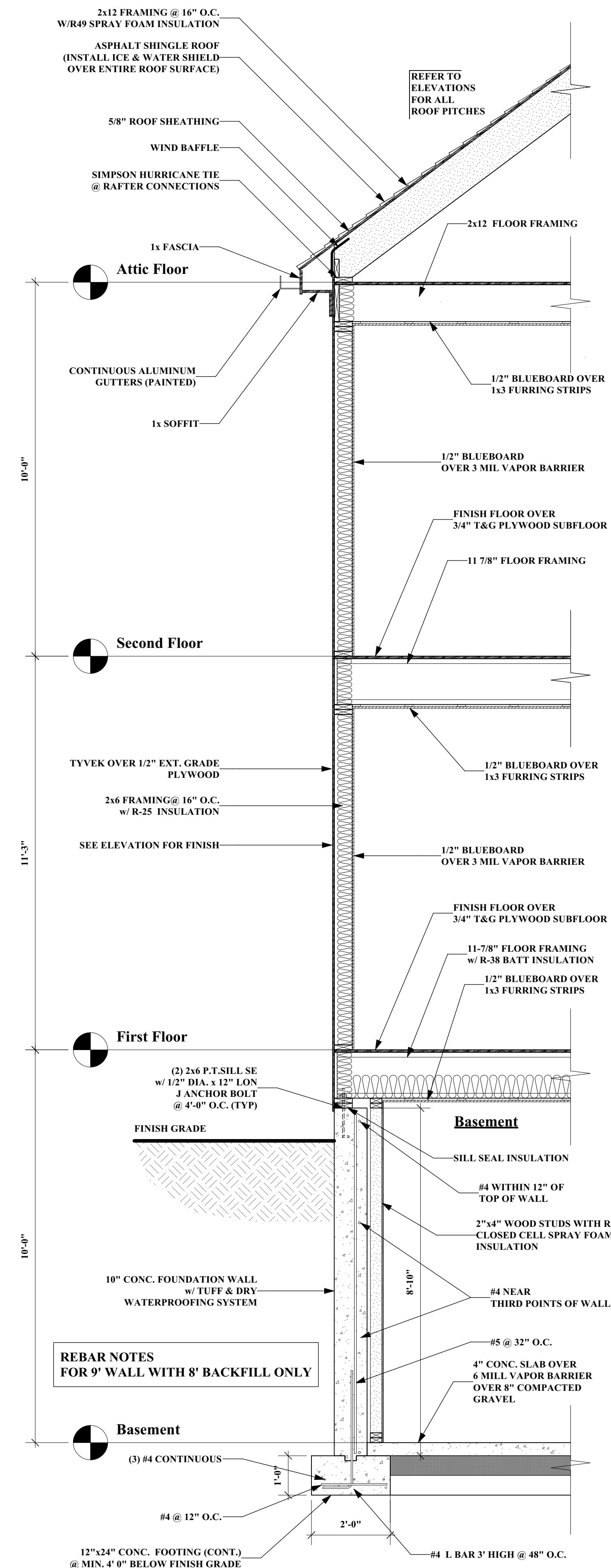
1 Typical Section A-3.1 1/2" = 1'-0"
